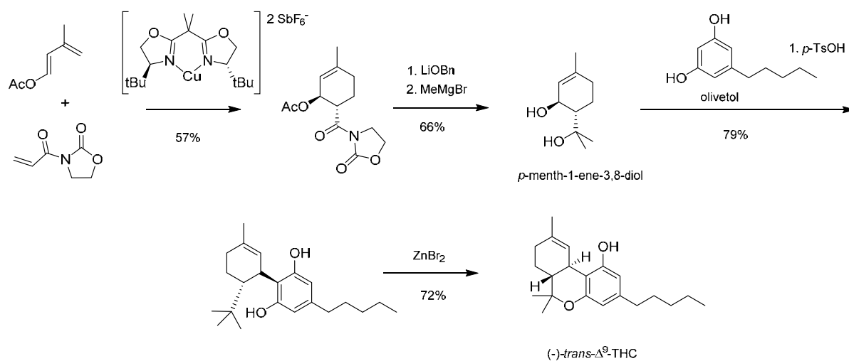
Fig. 11 Synthesis of (+)-trans- \Delta^9 -THC by Evans et al.
