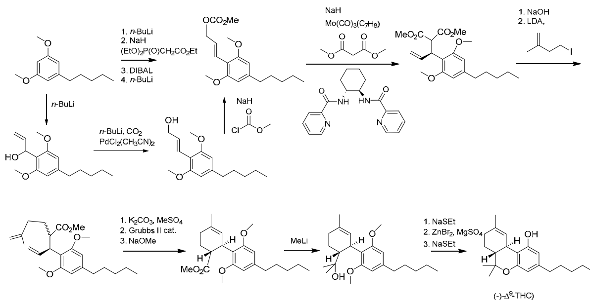
Fig. 12 Synthesis of (-)- \Delta^9 -THC by Trost et al.
