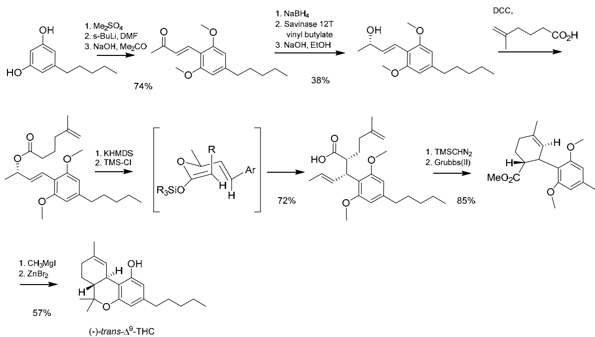
Fig. 16 Synthesis of (-)-Δ 9 -THC by Leahy et al.
