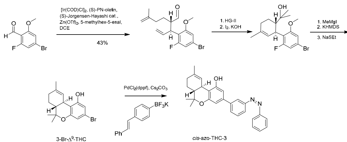
Fig. 15 Synthesis of azo-THC by Westphal et al.
