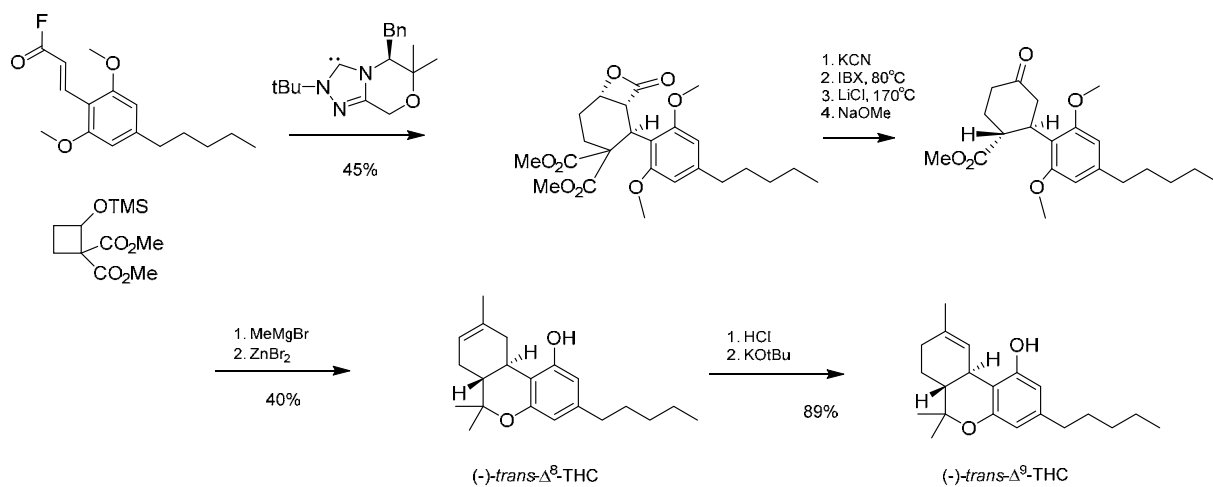
Fig. 17 Synthesis of (-)-Δ 9 -THC by Lupton et al.
