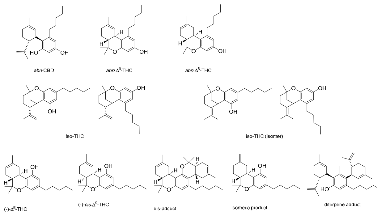
Fig. 6 By-products detected in the condensation of olivetol with monoterpenes
