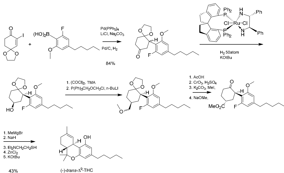
Fig. 14 Synthesis of (-)-Δ 9 -THC by Cheng et al.
